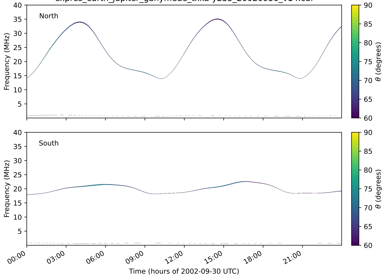
expres_earth_jupiter_ganymede_txka-y235_20020930_v14.cdf
