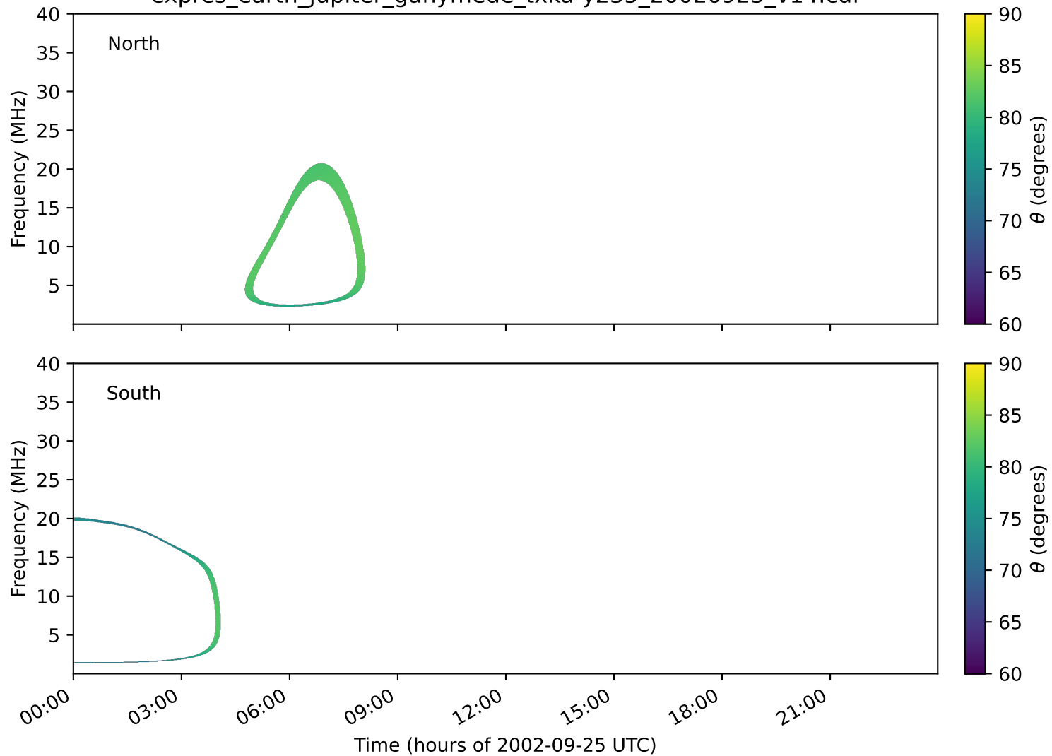
expres_earth_jupiter_ganymede_txka-y235_20020925_v14.cdf
