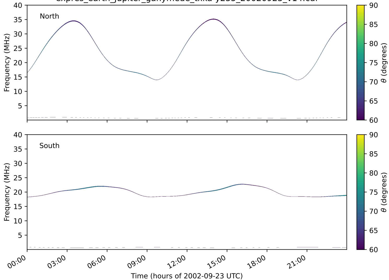
expres_earth_jupiter_ganymede_txka-y235_20020923_v14.cdf
