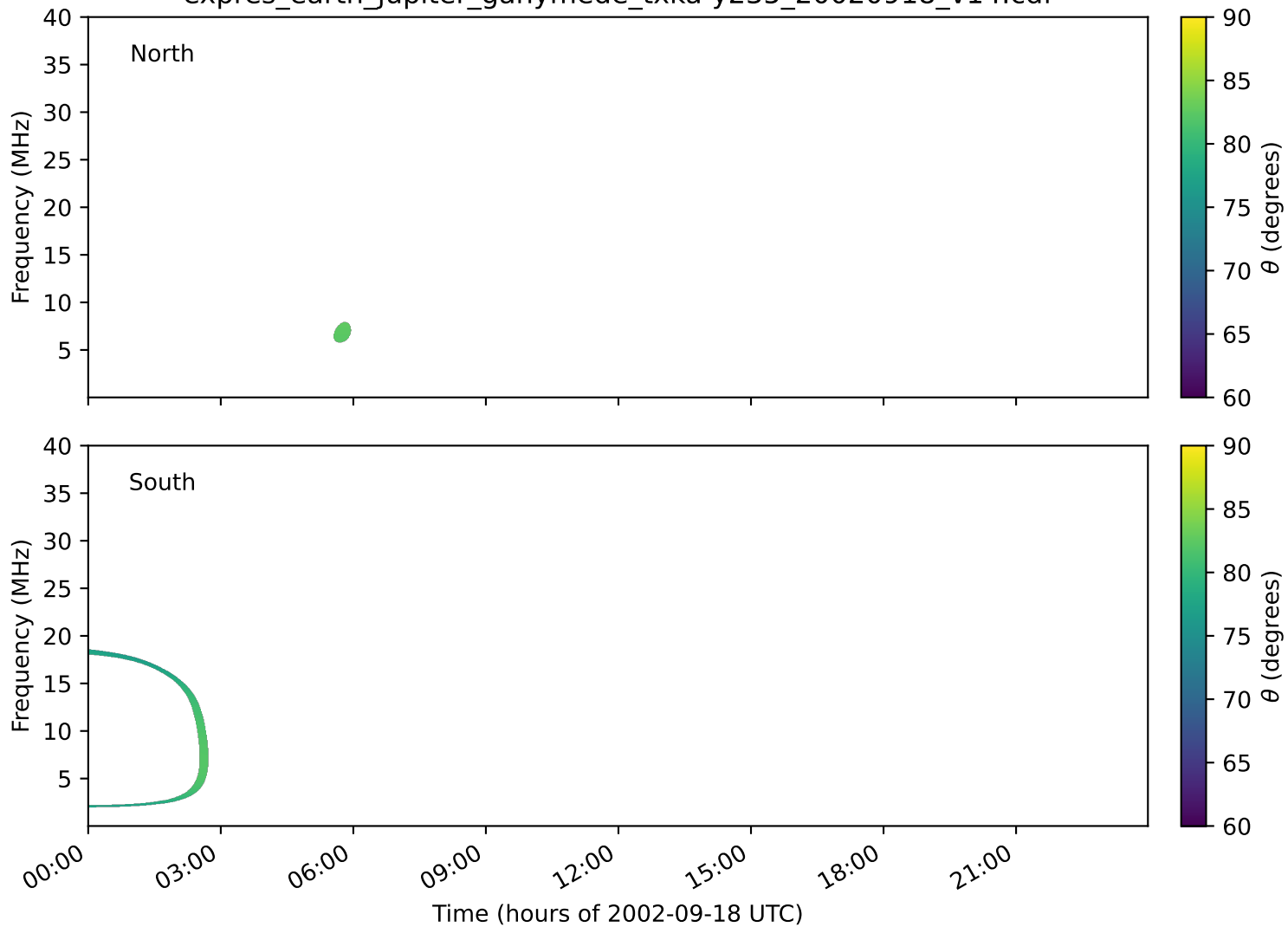
expres_earth_jupiter_ganymede_txka-y235_20020918_v14.cdf
