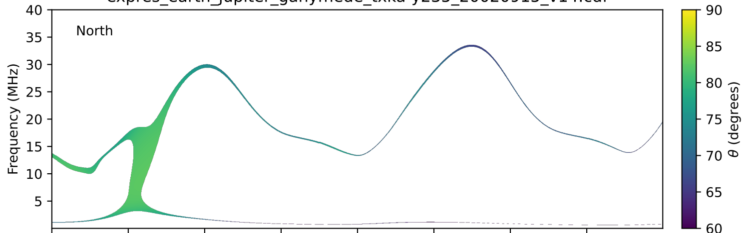
expres_earth_jupiter_ganymede_txka-y235_20020915_v14.cdf
