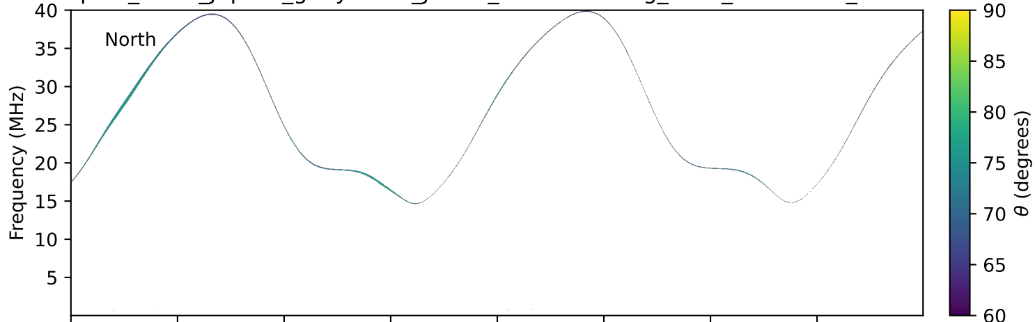
expres_earth_jupiter_ganymede_jrm33_lossc-wid1deg_3kev_20020930_v11.cdf
