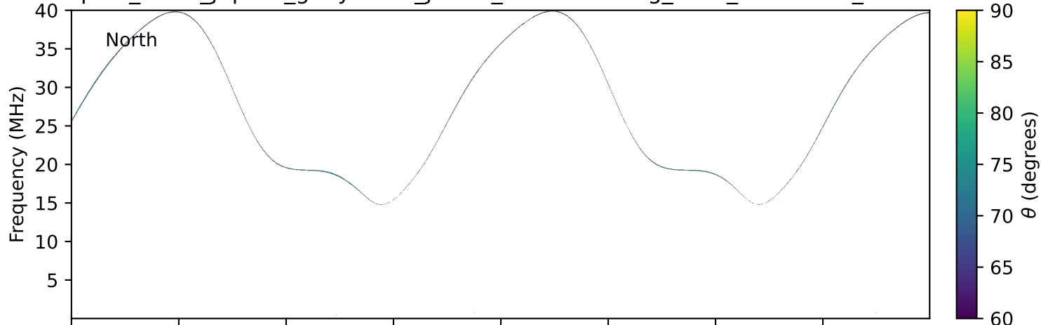
expres_earth_jupiter_ganymede_jrm33_lossc-wid1deg_3kev_20020916_v11.cdf
