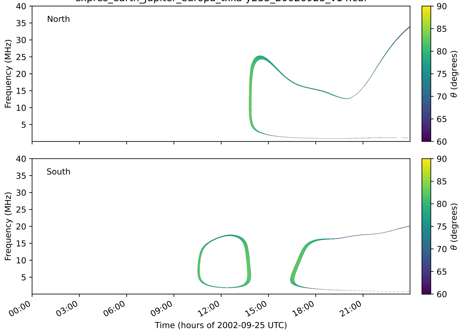
expres_earth_jupiter_europa_txka-y235_20020925_v14.cdf
