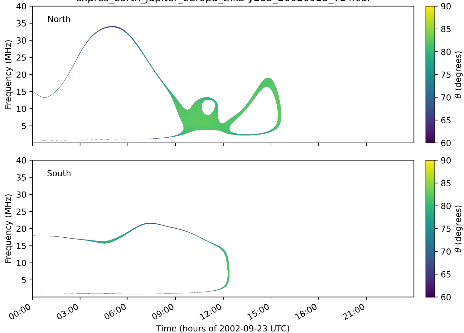
expres_earth_jupiter_europa_txka-y235_20020923_v14.cdf
