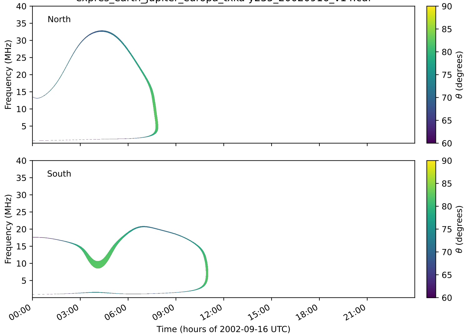
expres_earth_jupiter_europa_txka-y235_20020916_v14.cdf
