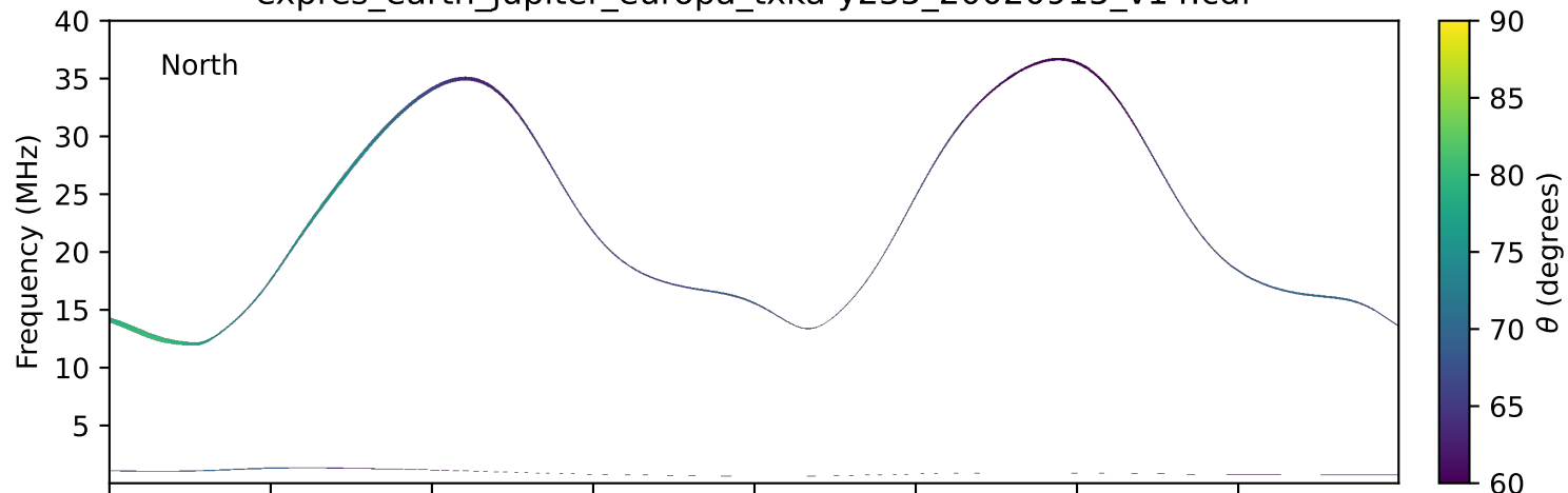
expres_earth_jupiter_europa_txka-y235_20020915_v14.cdf
