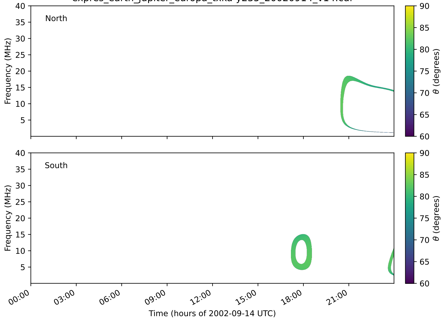
expres_earth_jupiter_europa_txka-y235_20020914_v14.cdf
