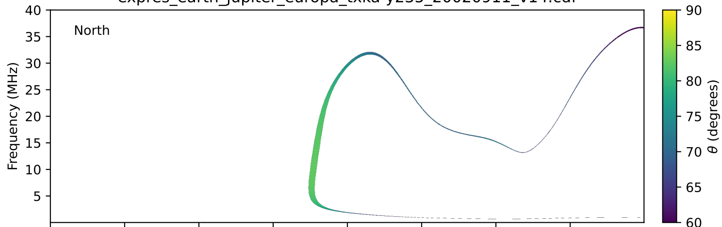
expres_earth_jupiter_europa_txka-y235_20020911_v14.cdf
