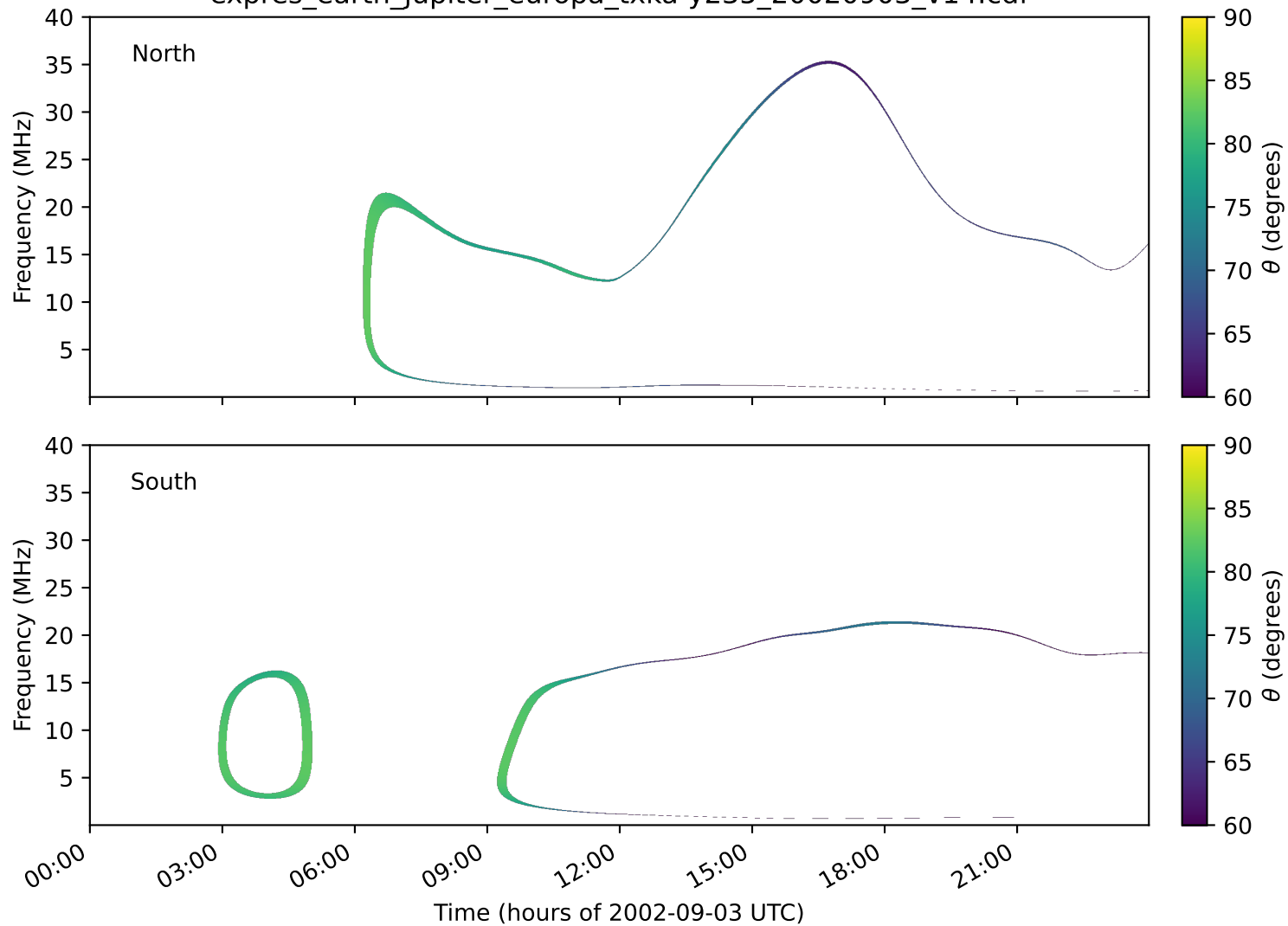
expres_earth_jupiter_europa_txka-y235_20020903_v14.cdf
