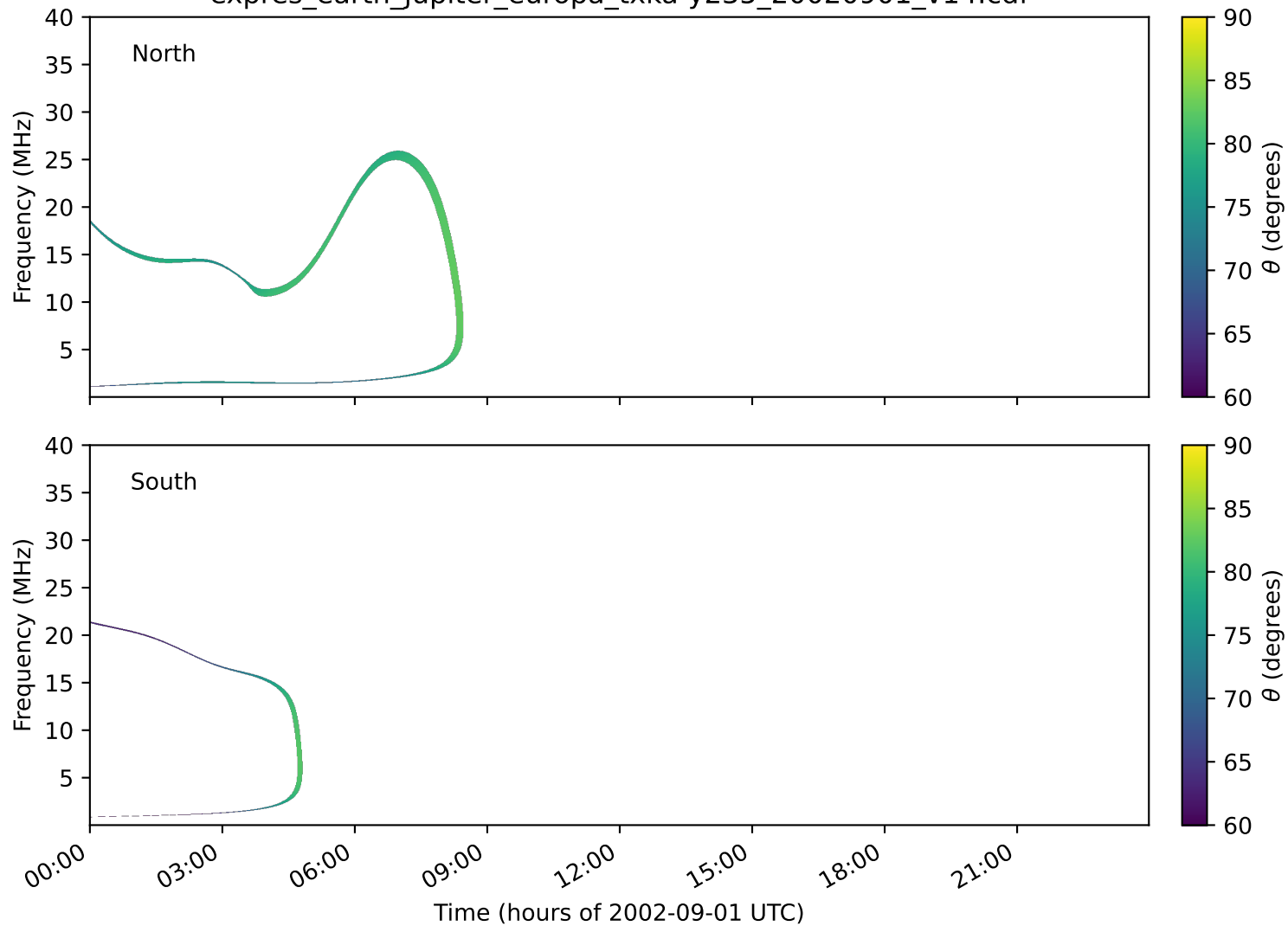
expres_earth_jupiter_europa_txka-y235_20020901_v14.cdf
