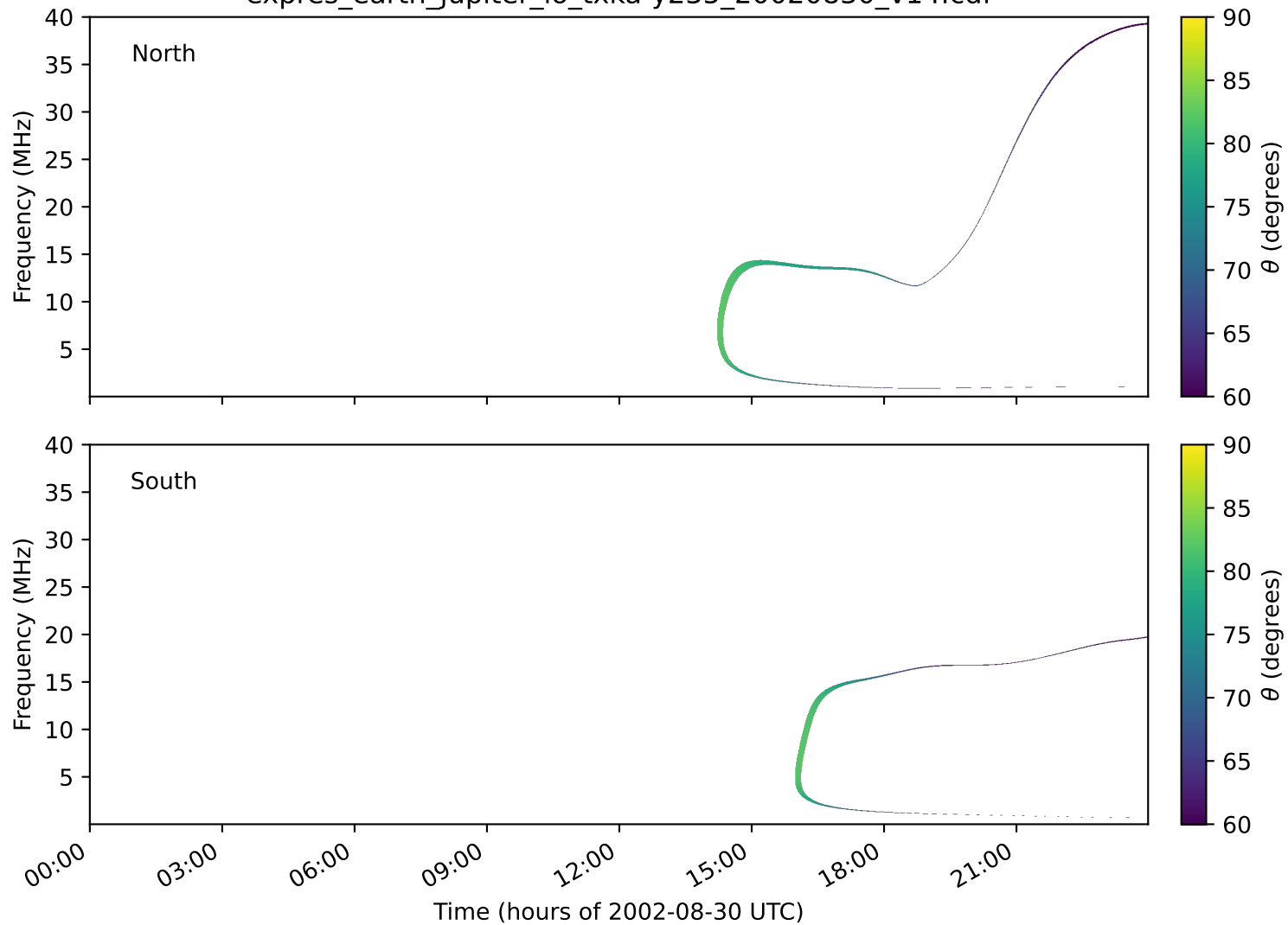
expres_earth_jupiter_io_txka-y235_20020830_v14.cdf
