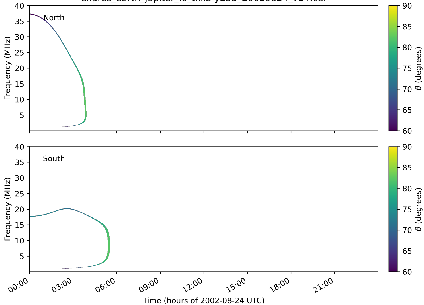
expres_earth_jupiter_io_txka-y235_20020824_v14.cdf
