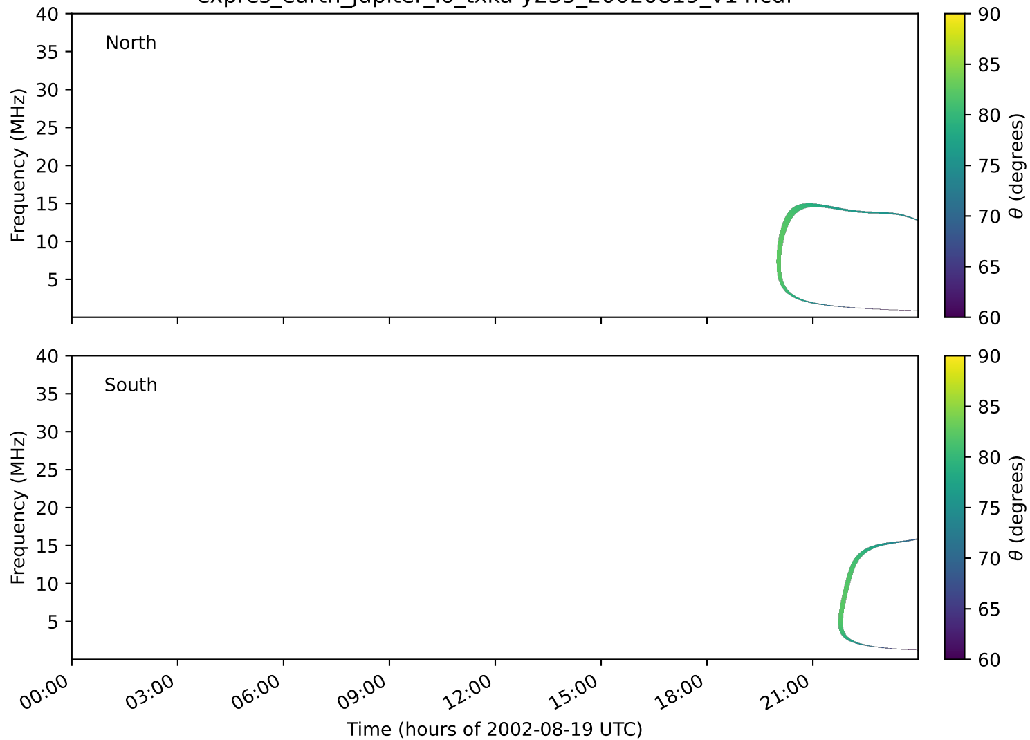
expres_earth_jupiter_io_txka-y235_20020819_v14.cdf
