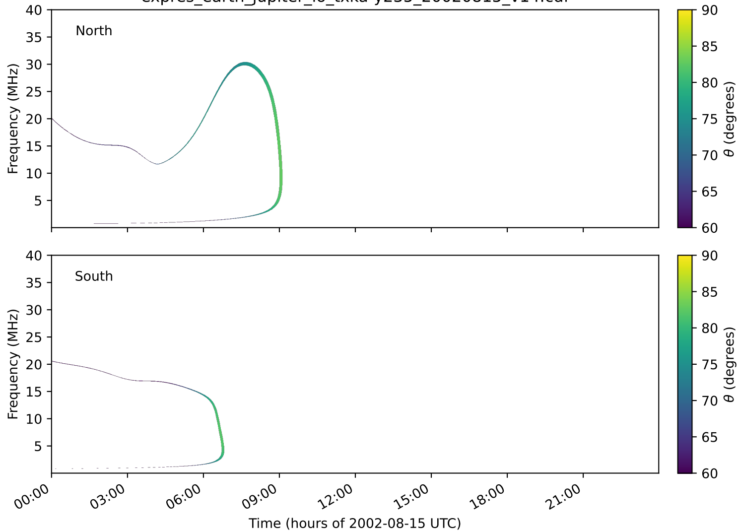
expres_earth_jupiter_io_txka-y235_20020815_v14.cdf
