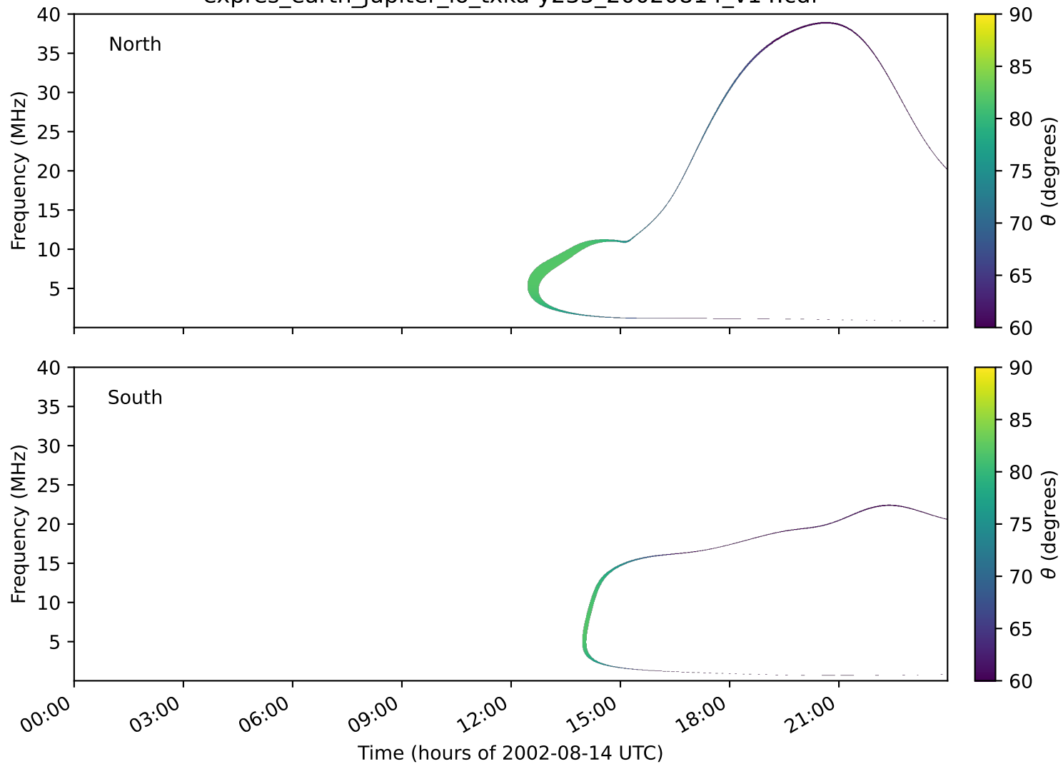
expres_earth_jupiter_io_txka-y235_20020814_v14.cdf
