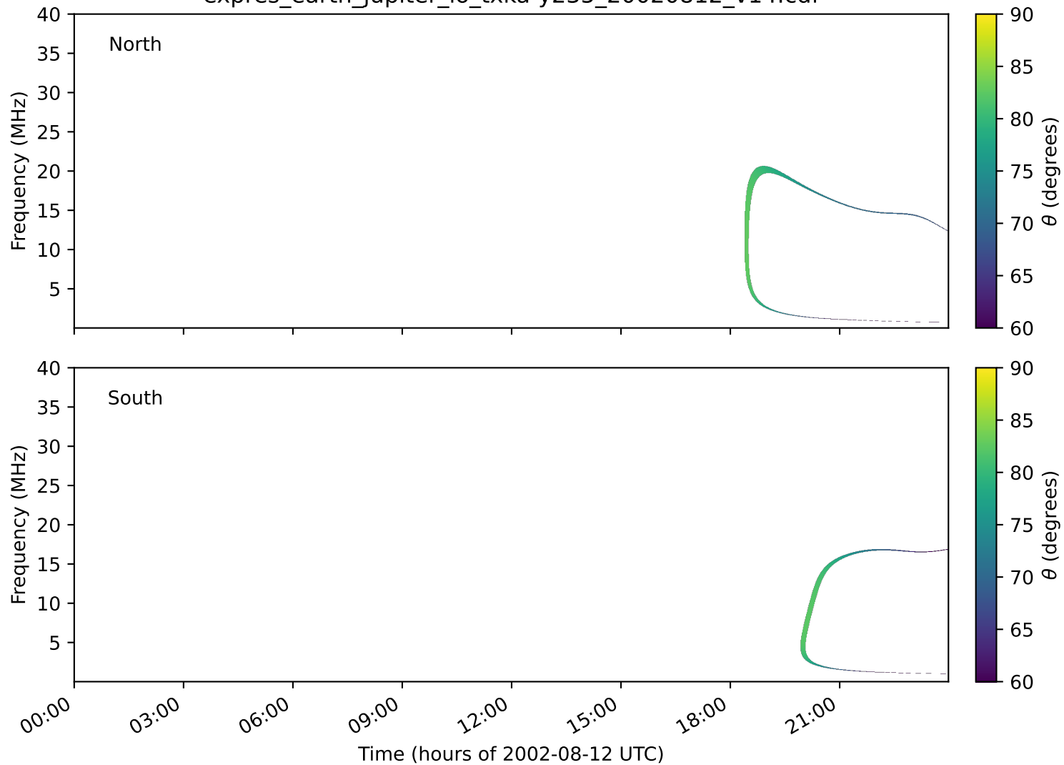
expres_earth_jupiter_io_txka-y235_20020812_v14.cdf
