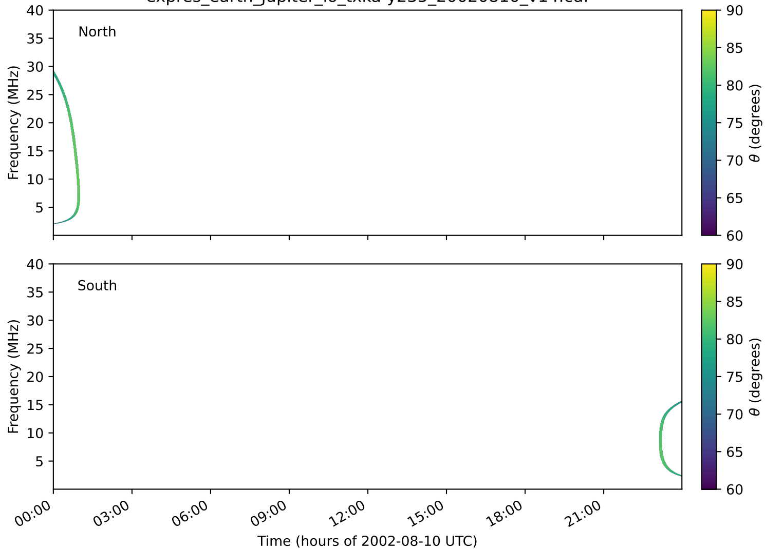
expres_earth_jupiter_io_txka-y235_20020810_v14.cdf
