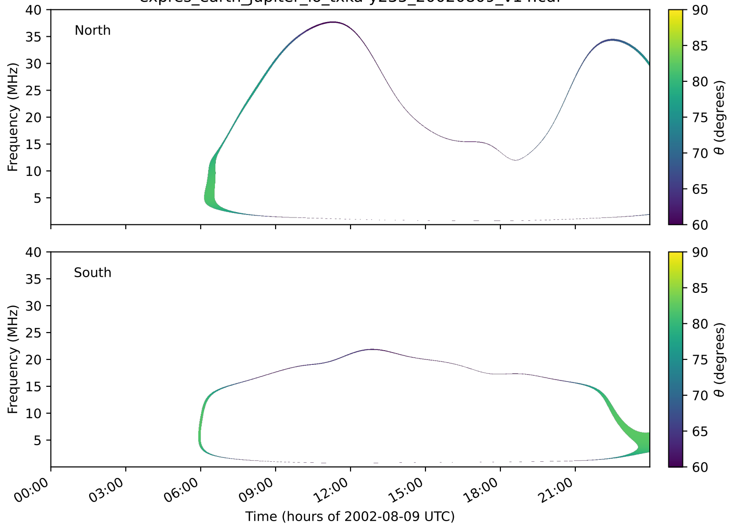
expres_earth_jupiter_io_txka-y235_20020809_v14.cdf
