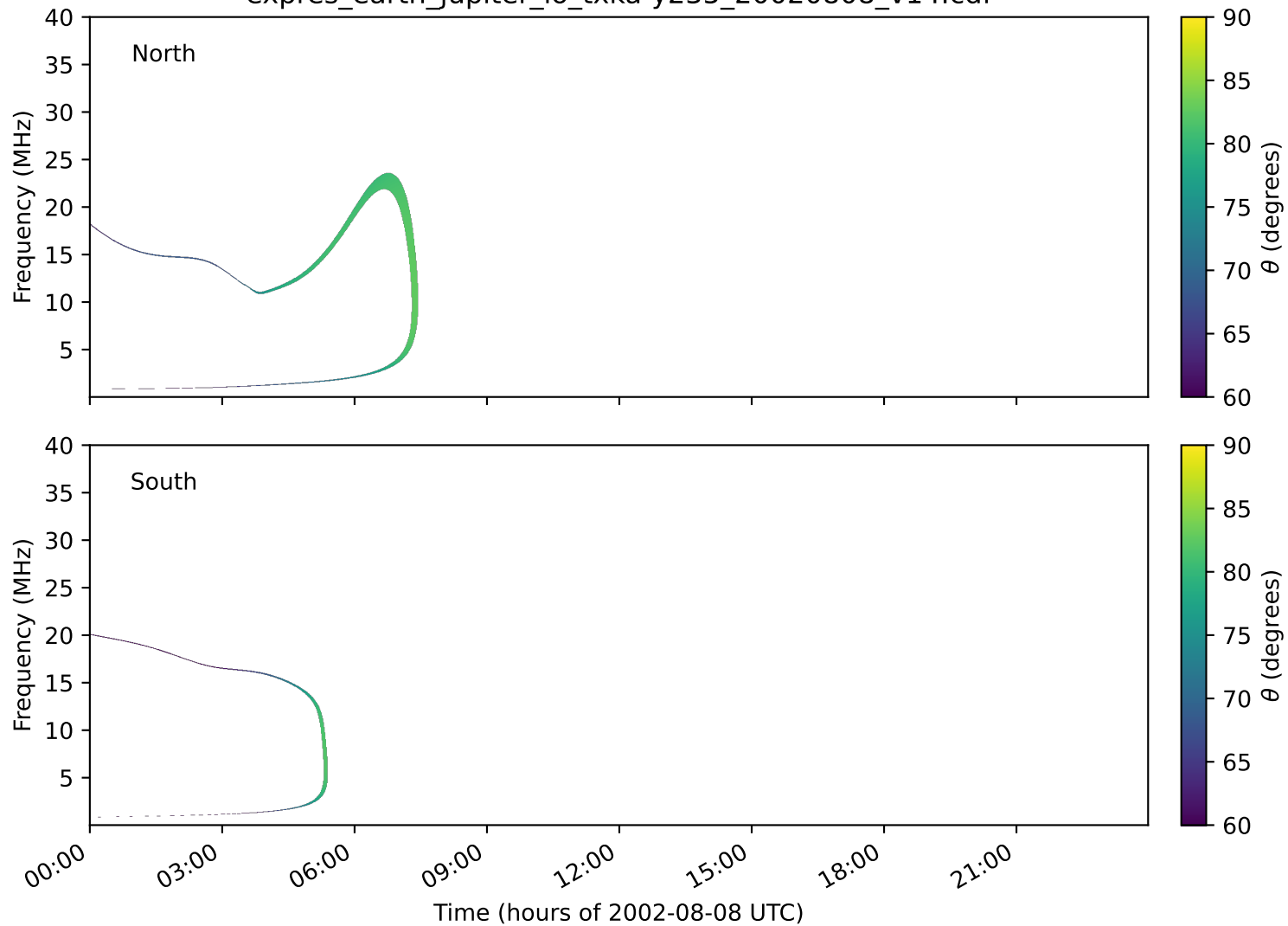
expres_earth_jupiter_io_txka-y235_20020808_v14.cdf
