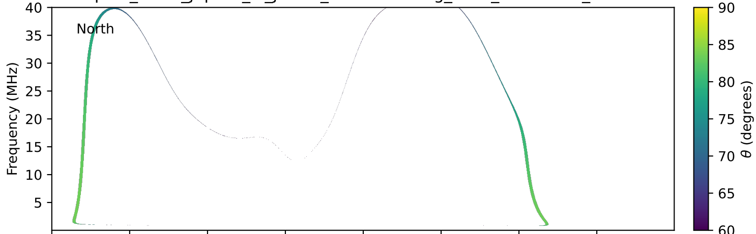
expres_earth_jupiter_io_jrm33_lossc-wid1deg_3kev_20020811_v11.cdf
