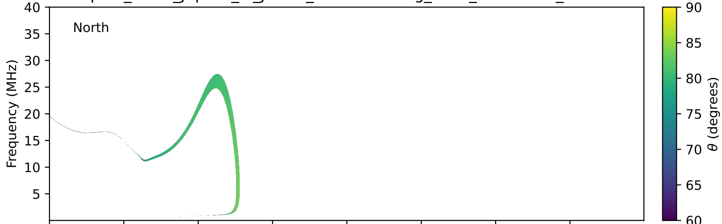
expres_earth_jupiter_io_jrm33_lossc-wid1deg_3kev_20020808_v11.cdf
