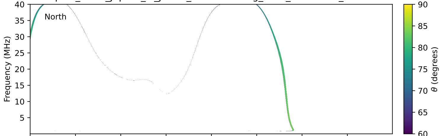
expres_earth_jupiter_io_jrm33_lossc-wid1deg_3kev_20020804_v11.cdf
