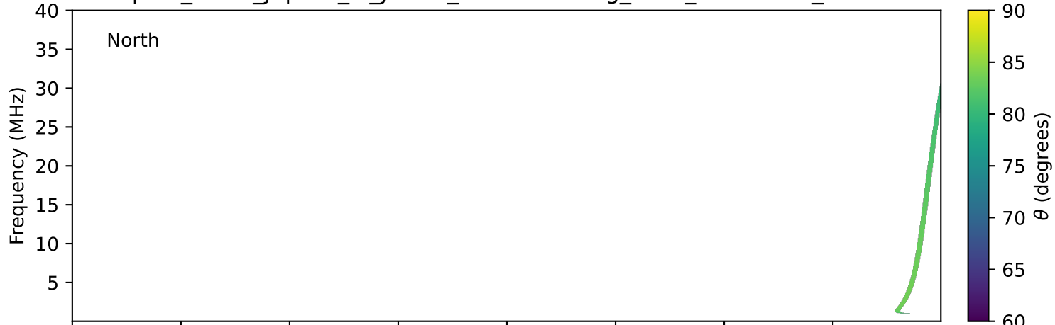
expres_earth_jupiter_io_jrm33_lossc-wid1deg_3kev_20020803_v11.cdf
