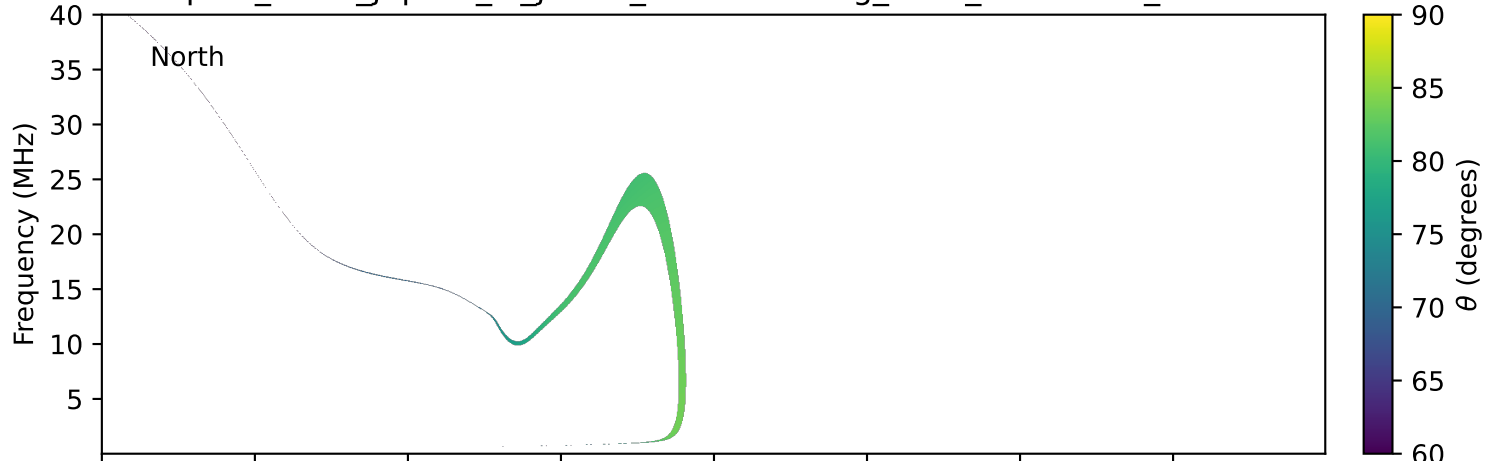
expres_earth_jupiter_io_jrm09_lossc-wid1deg_3kev_20020831_v11.cdf
