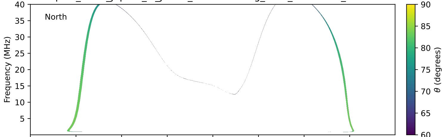
expres_earth_jupiter_io_jrm09_lossc-wid1deg_3kev_20020827_v11.cdf
