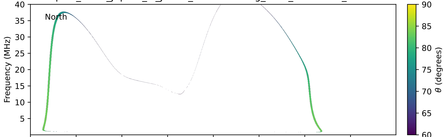
expres_earth_jupiter_io_jrm09_lossc-wid1deg_3kev_20020811_v11.cdf
