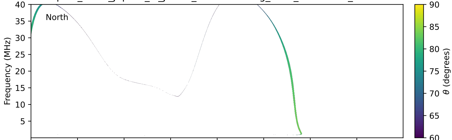
expres_earth_jupiter_io_jrm09_lossc-wid1deg_3kev_20020804_v11.cdf
