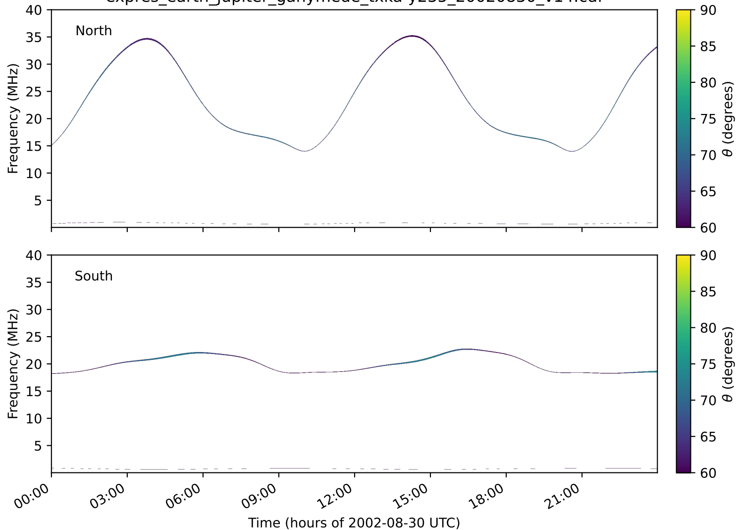
expres_earth_jupiter_ganymede_txka-y235_20020830_v14.cdf
