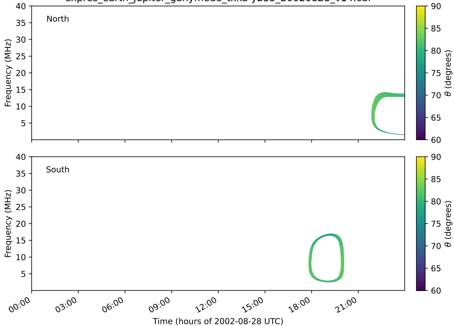
expres_earth_jupiter_ganymede_txka-y235_20020828_v14.cdf
