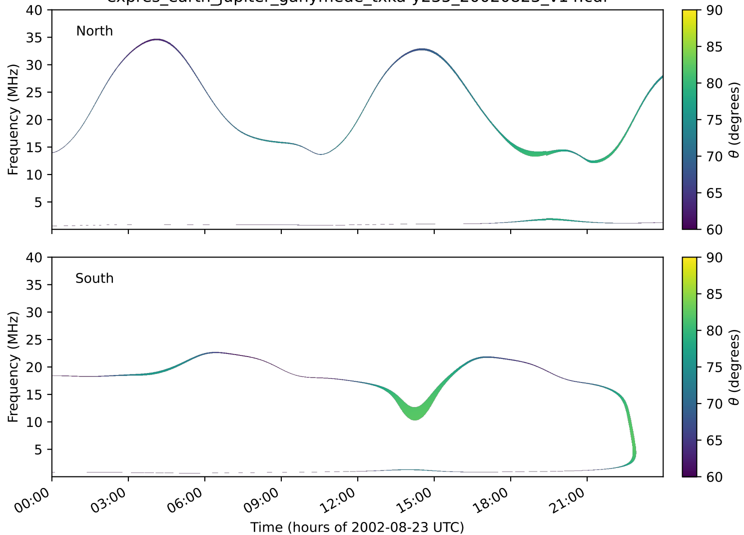
expres_earth_jupiter_ganymede_txka-y235_20020823_v14.cdf
