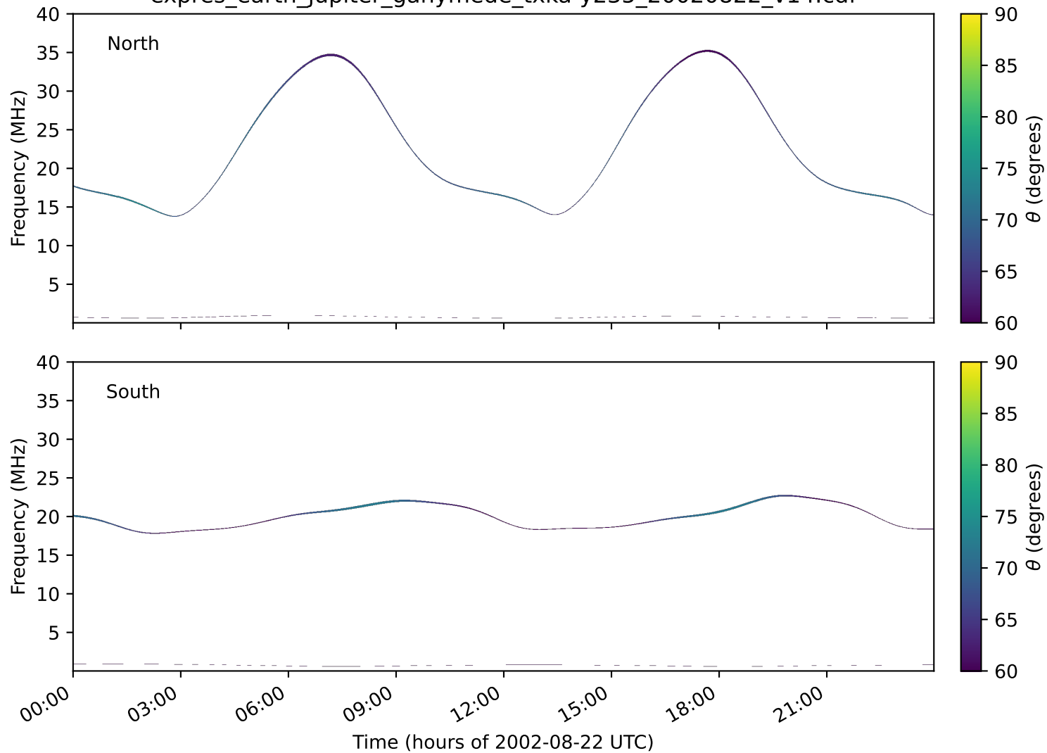
expres_earth_jupiter_ganymede_txka-y235_20020822_v14.cdf
