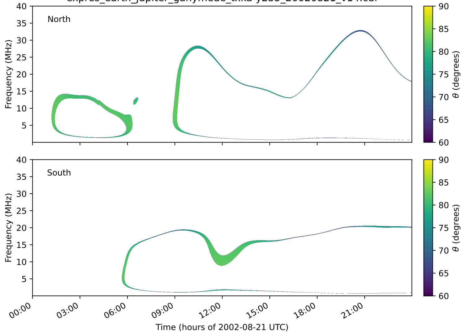
expres_earth_jupiter_ganymede_txka-y235_20020821_v14.cdf
