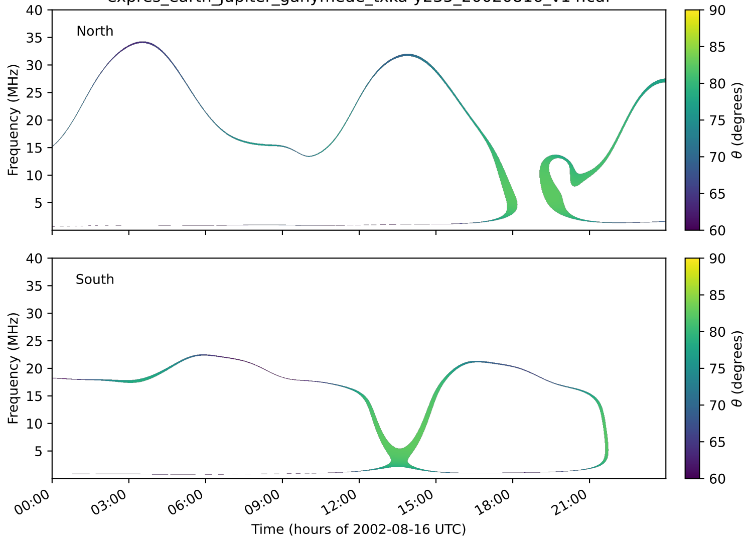
expres_earth_jupiter_ganymede_txka-y235_20020816_v14.cdf
