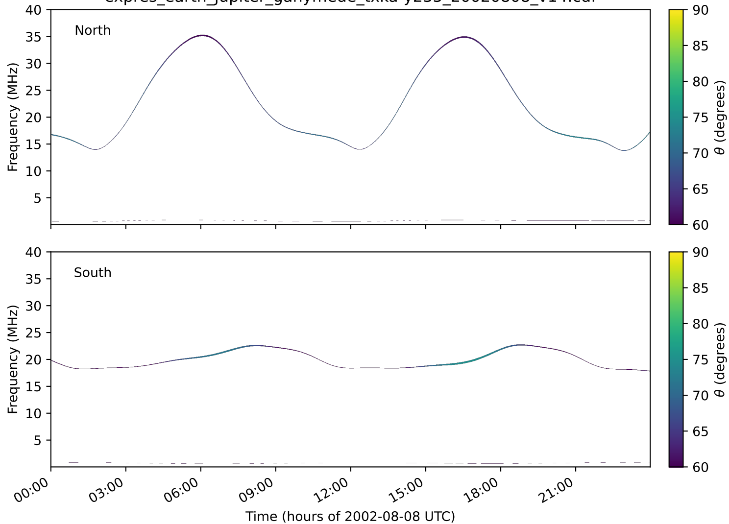
expres_earth_jupiter_ganymede_txka-y235_20020808_v14.cdf
