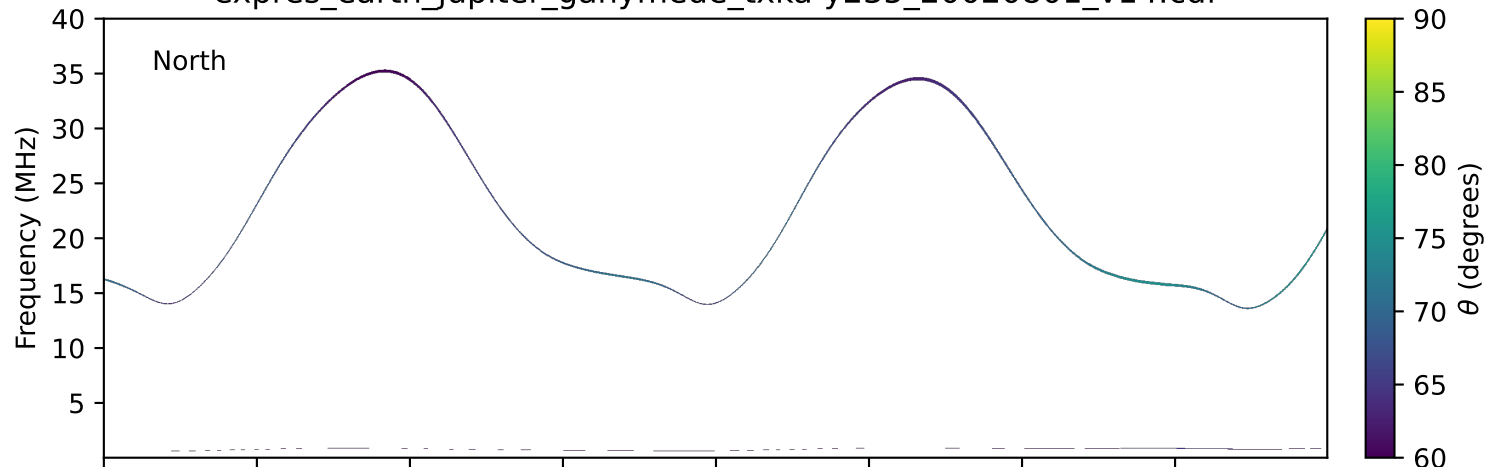
expres_earth_jupiter_ganymede_txka-y235_20020801_v14.cdf
