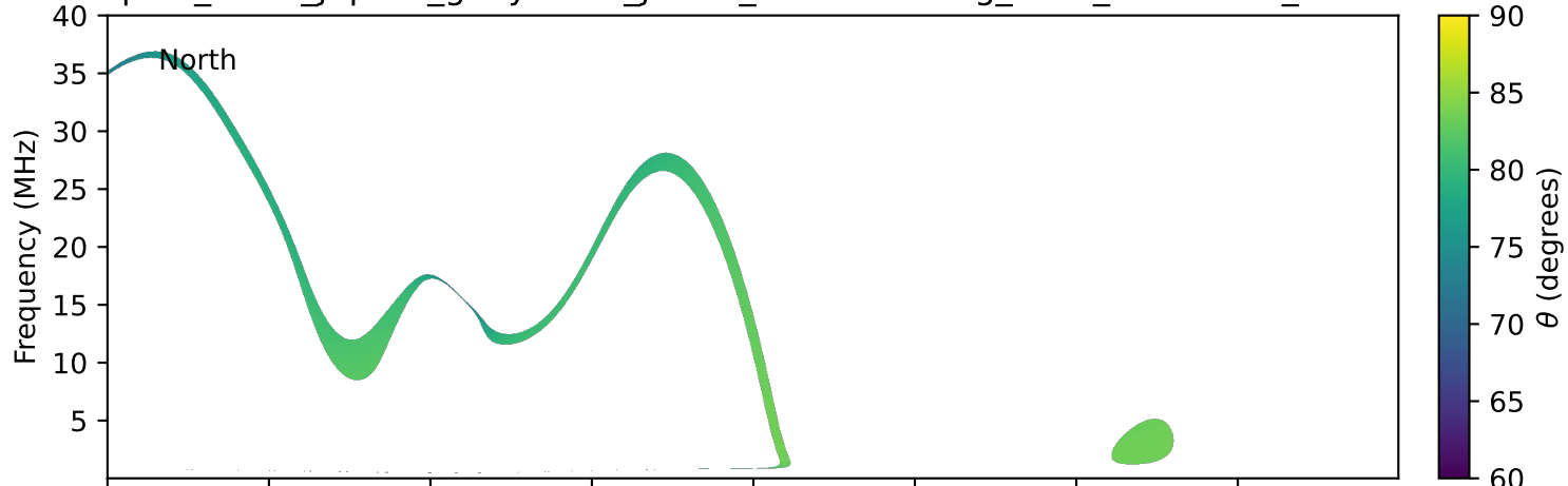
expres_earth_jupiter_ganymede_jrm33_lossc-wid1deg_3kev_20020824_v11.cdf
