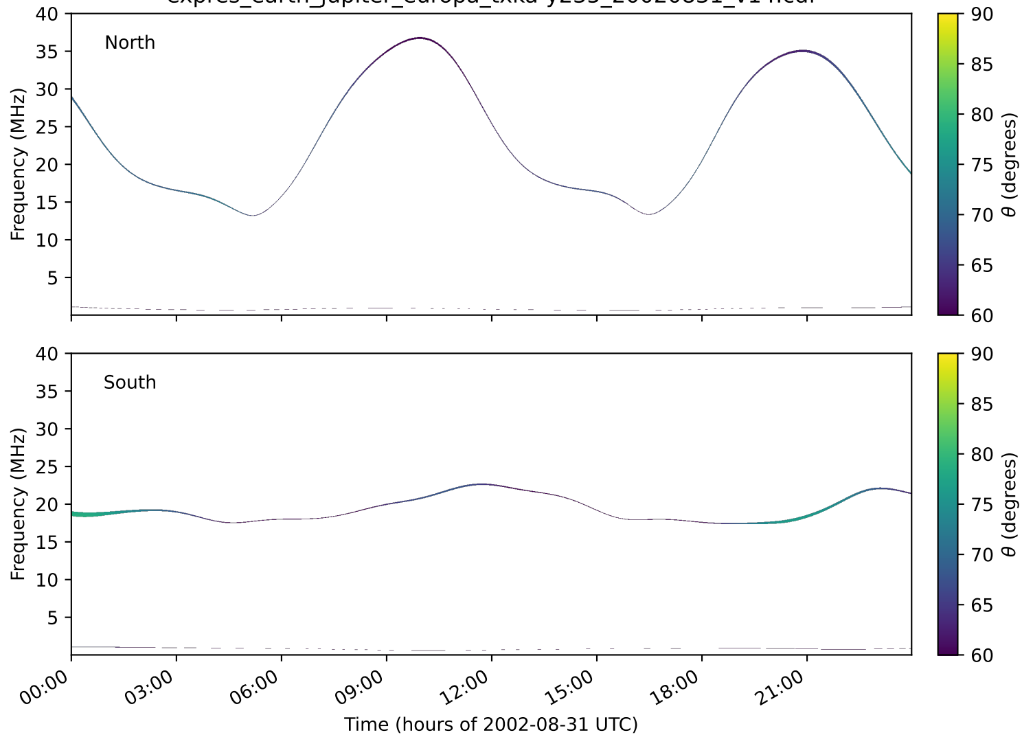
expres_earth_jupiter_europa_txka-y235_20020831_v14.cdf
