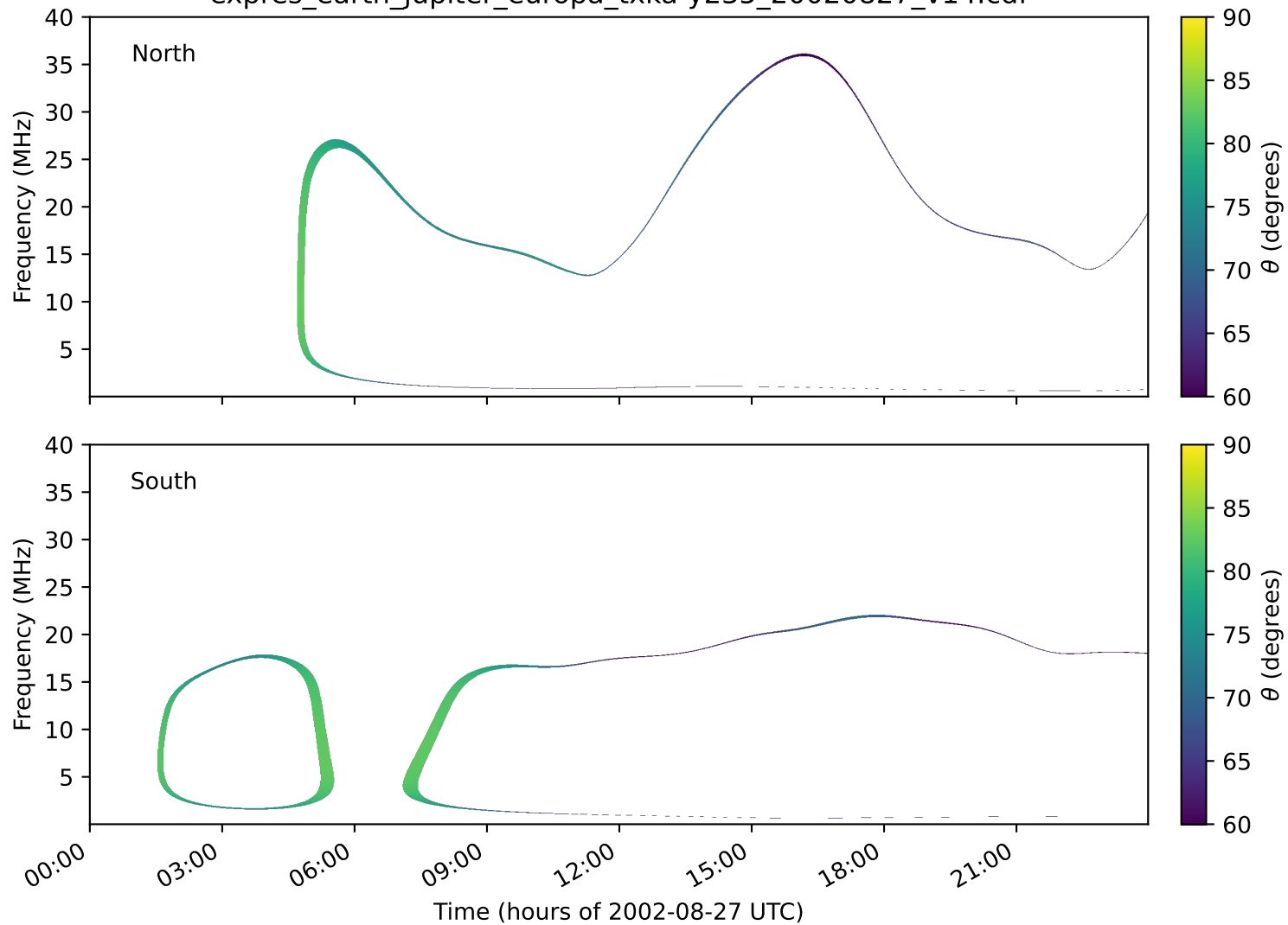
expres_earth_jupiter_europa_txka-y235_20020827_v14.cdf
