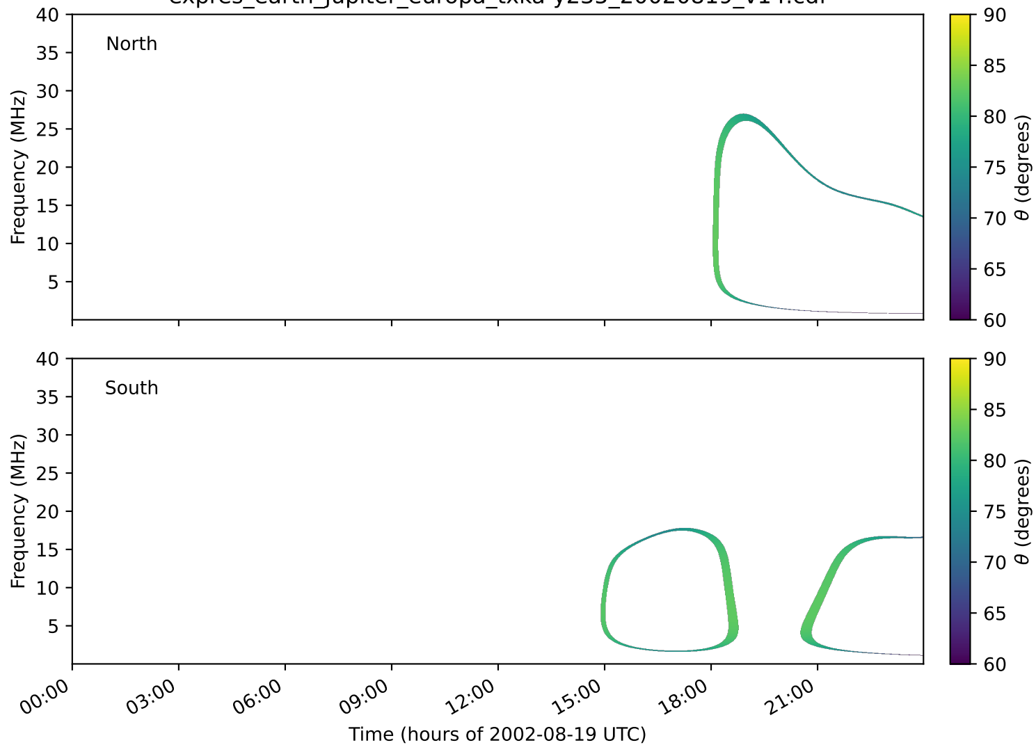
expres_earth_jupiter_europa_txka-y235_20020819_v14.cdf
