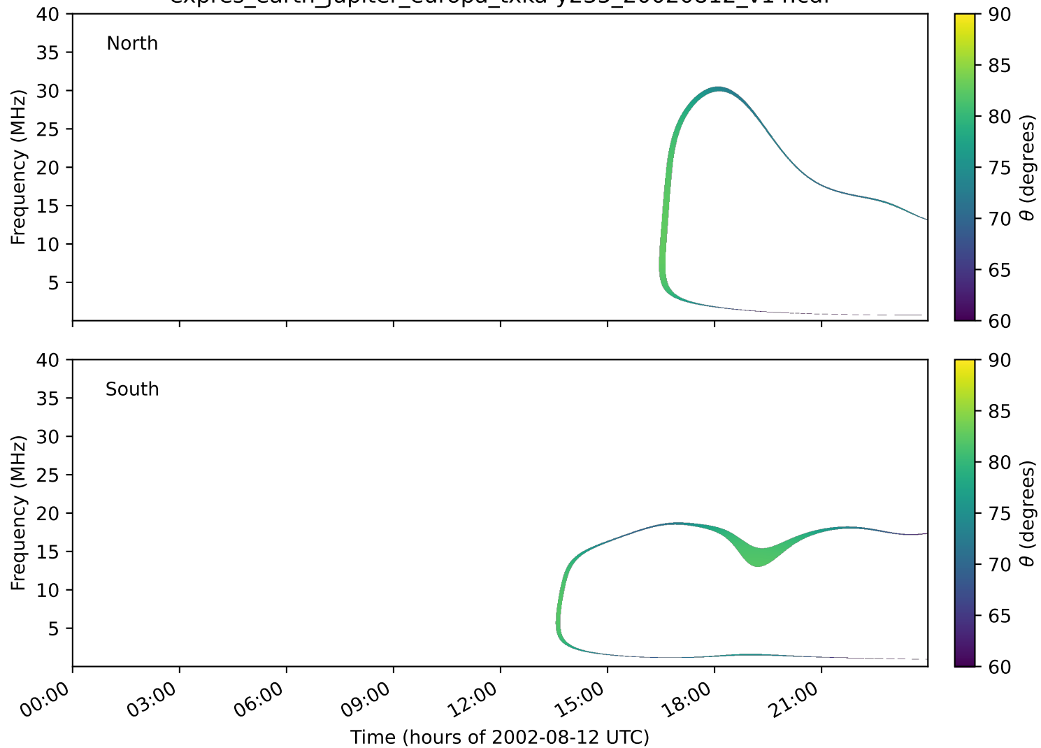
expres_earth_jupiter_europa_txka-y235_20020812_v14.cdf
