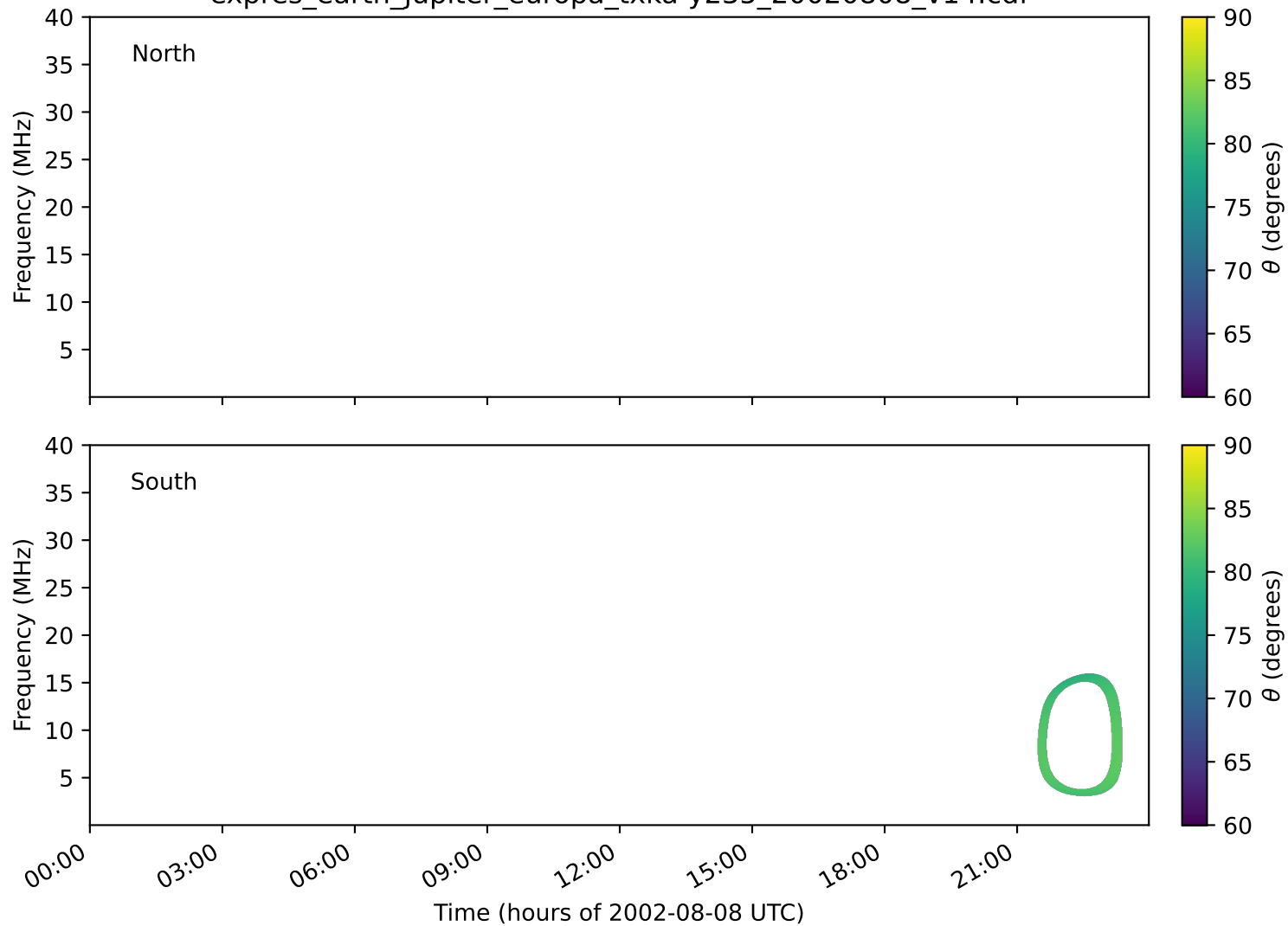
expres_earth_jupiter_europa_txka-y235_20020808_v14.cdf
