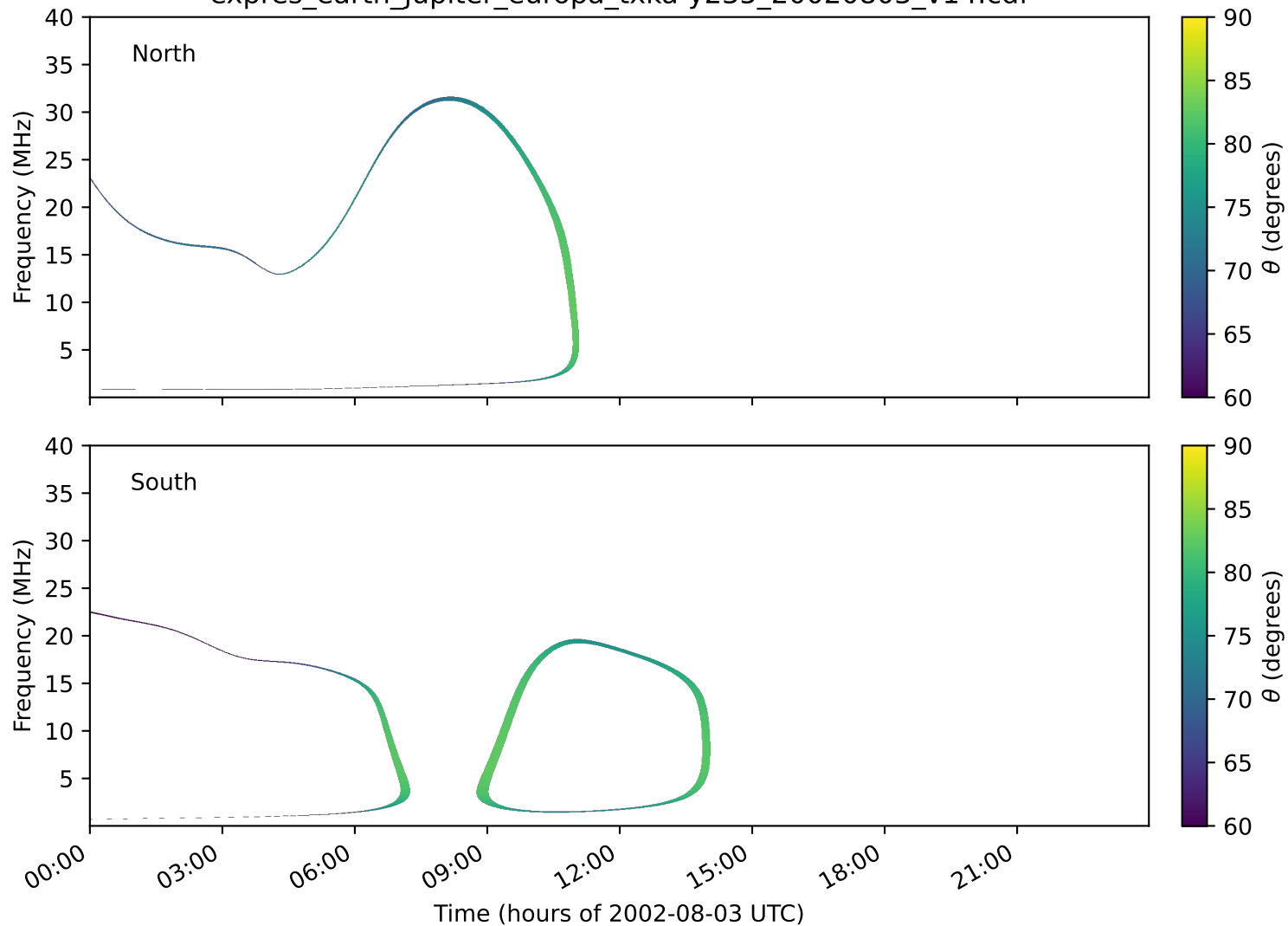
expres_earth_jupiter_europa_txka-y235_20020803_v14.cdf
