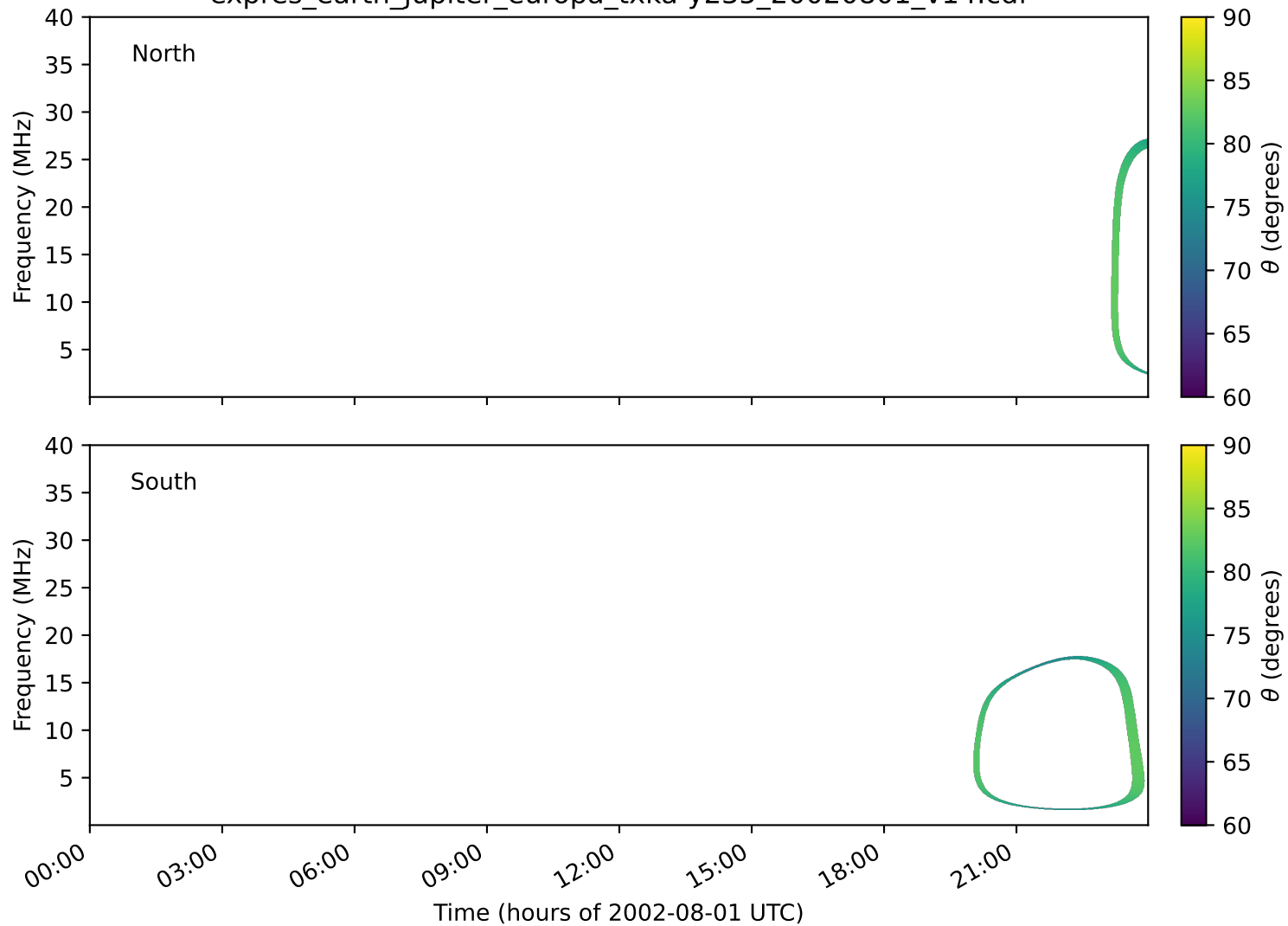
expres_earth_jupiter_europa_txka-y235_20020801_v14.cdf
