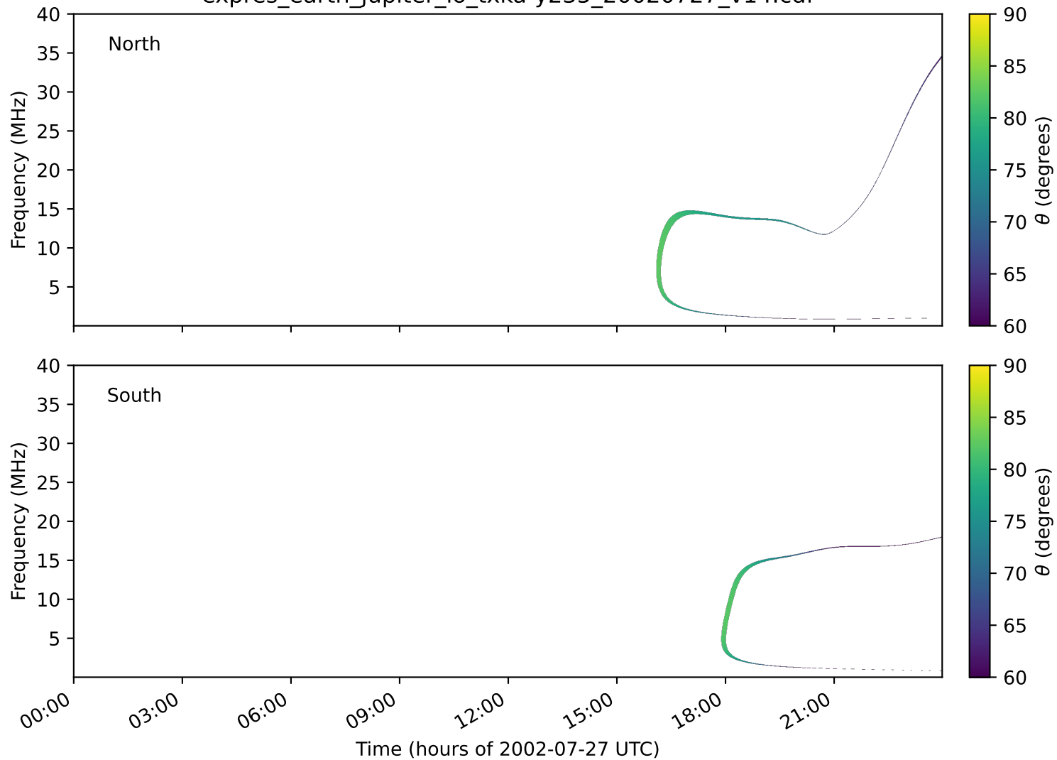
expres_earth_jupiter_io_txka-y235_20020727_v14.cdf
