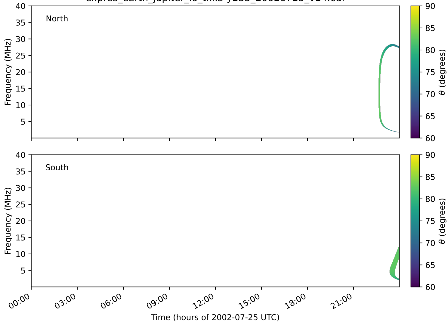
expres_earth_jupiter_io_txka-y235_20020725_v14.cdf
